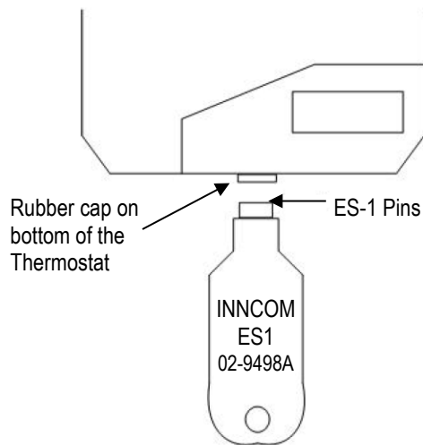
Figure 2. Connecting the ES-1 to the Thermostat
